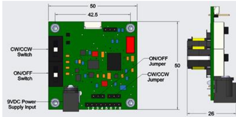
BOARD DIMENSIONS
